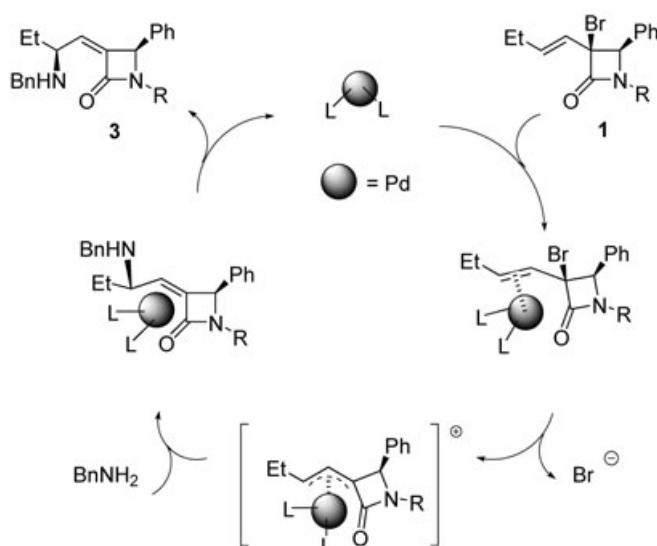
Figure 1. Mechanism suggested for the palladium-catalyzed addition of benzylamine.
