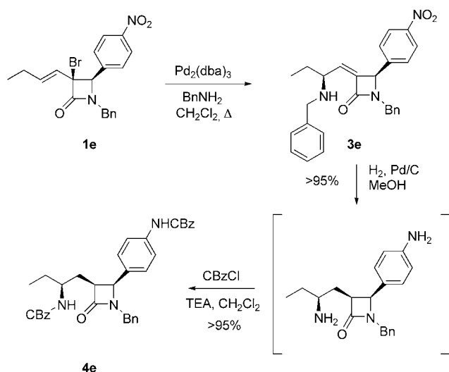
Scheme 3. Synthesis of 3-(2'-CBz-amino)-azetidin-2-one 4e .
