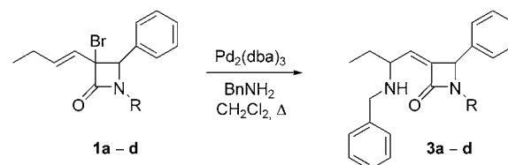
Scheme 2. Palladium-catalyzed benzylamine attack to 1a–d .
