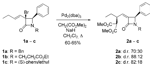
Scheme 1. Allylic alkylation of 1a–c with dimethyl malonate.
