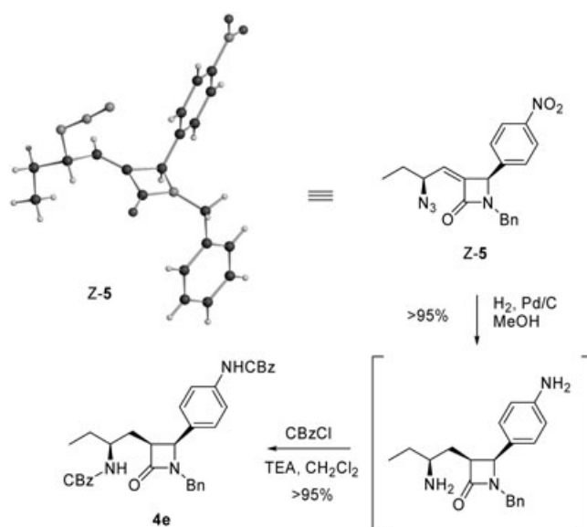
Scheme 4. Synthesis of 3-(2'-CBz-amino)-azetidin-2-one 4e , starting from azide 5 .
