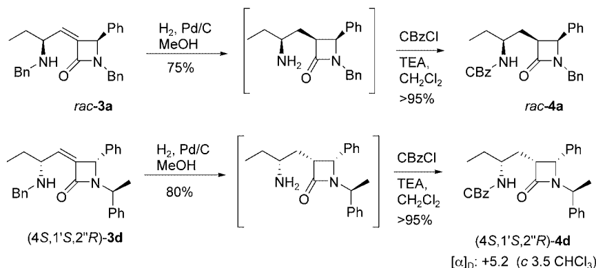
Scheme 5. Synthesis of 3-(2'-CBz-amino)-azetidin-2-ones 4a – d .
